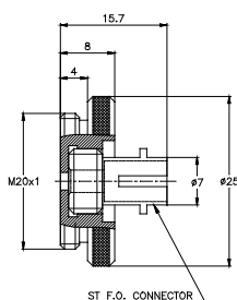
ST fiber adapter
