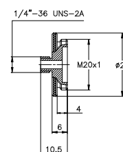
SM1 to M20 Adapter Mounting Bracket for PD300R Series and FPS-1, P/N 1G02259
