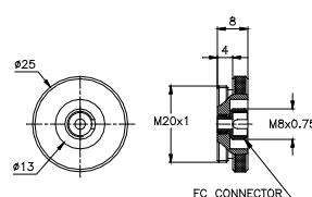
FC fiber adapter
