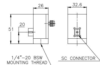
PD300-FO-SC
