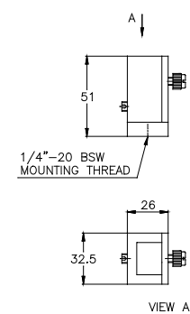
PD300-FO-FC
