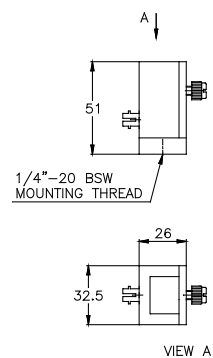
PD300-FO-ST
