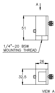
PD300-FO-SC
